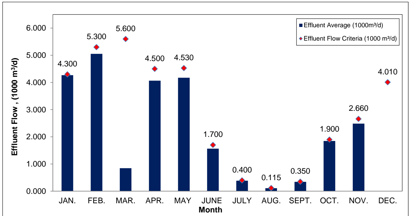
Tavistock WWTP Effluent, Monthly Average Daily Flow (1000 m 3 ), 2023
