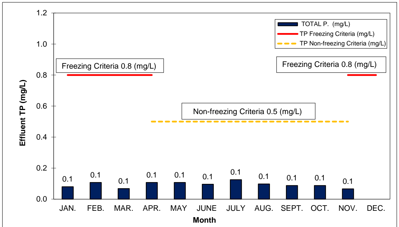
Tavistock WWTP Effluent, Monthly Average Total Phosphorus (mg/L), 2023
